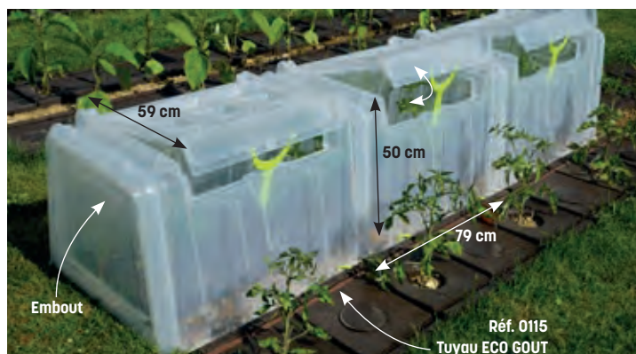
Tuyau ECO GOUT
